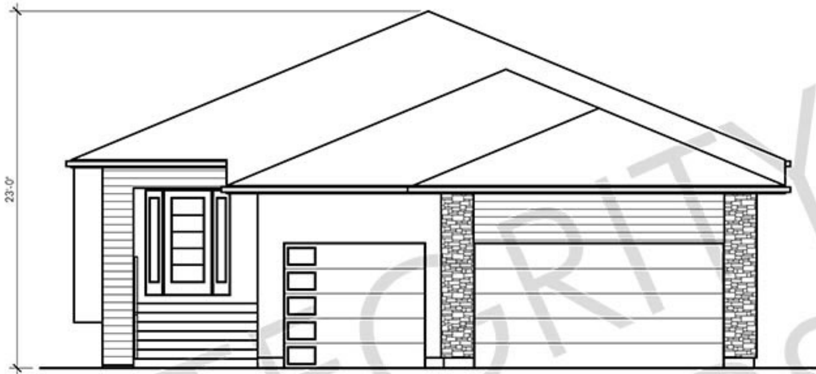
FRONT ELEVATION BIRCHWOOD-1440
