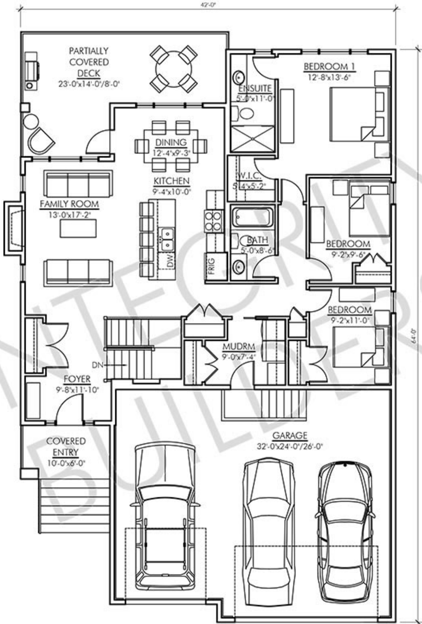
MAIN FLOOR PLAN - 1440 SQ FT BIRCHWOOD-1440
